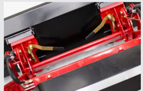
Quick attach skid steer style loader couplers are standard on all 4500 series loaders for ultra-fast front implement attachment.
